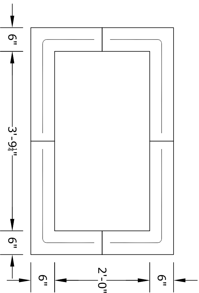
ASSEMBLY VIEW
